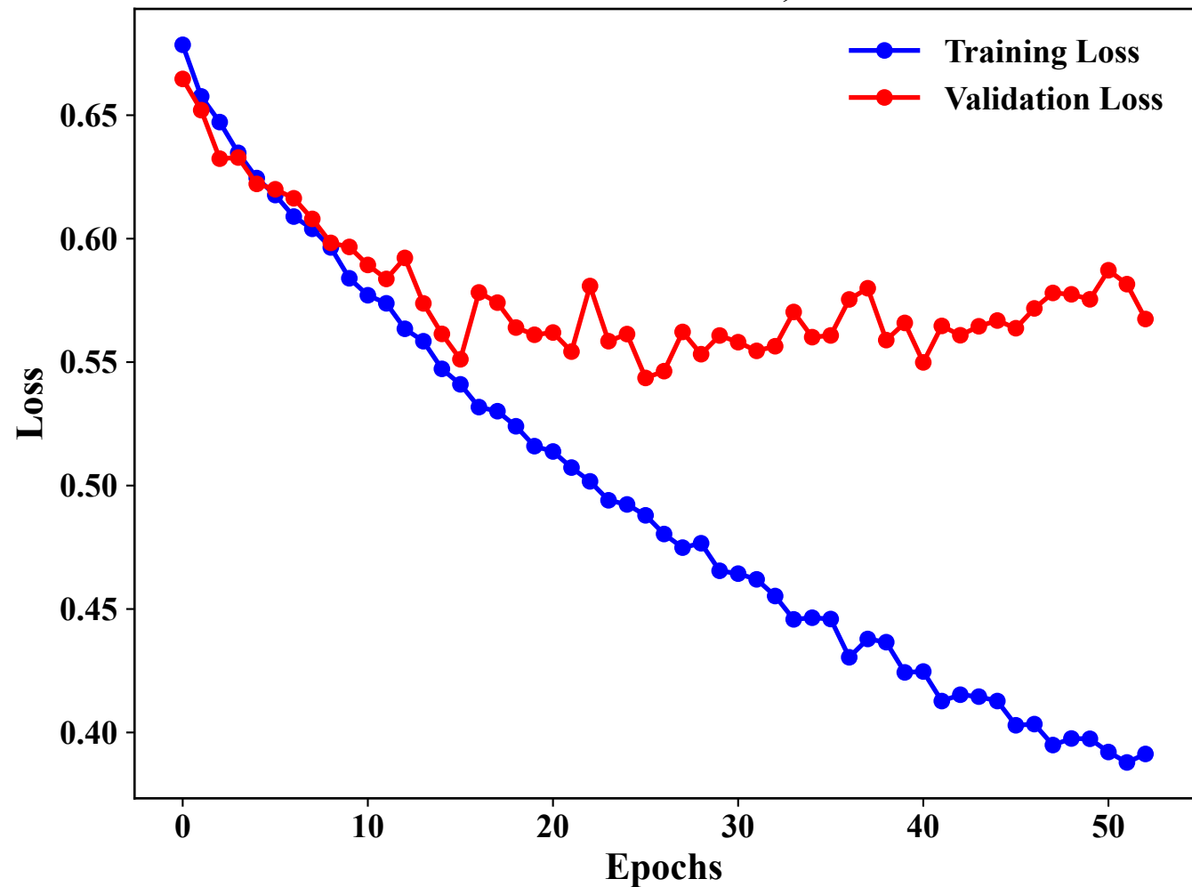
Loss Curves: Seed 48, Rank 1
